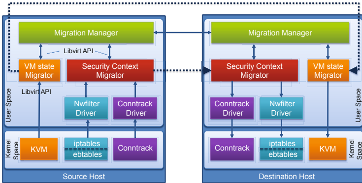
Fig. 5. SCM Framework Implementation
