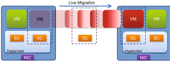
Fig. 1. Security Context Migration (SCM) Principle
