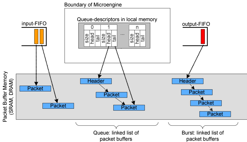
Fig. 5. Queueing and assembly using linked lists of packet buffers
