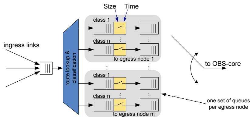
Fig. 2. Burst Assembly Unit for n traffic classes and m egress nodes
