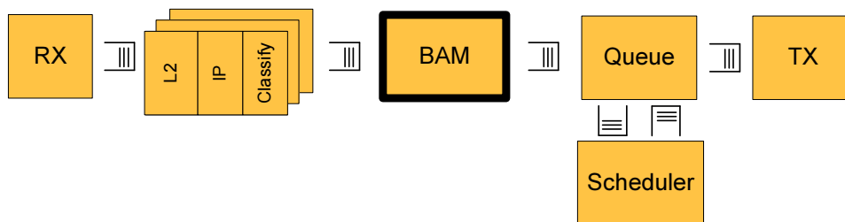
Fig. 6. Integration of the BAM into the BAU
