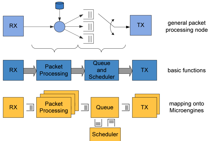
Fig. 4. Mapping of functions to microengines as defined by the software framework
