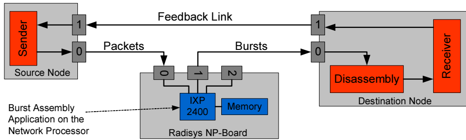
Fig. 7. Setup for testing
