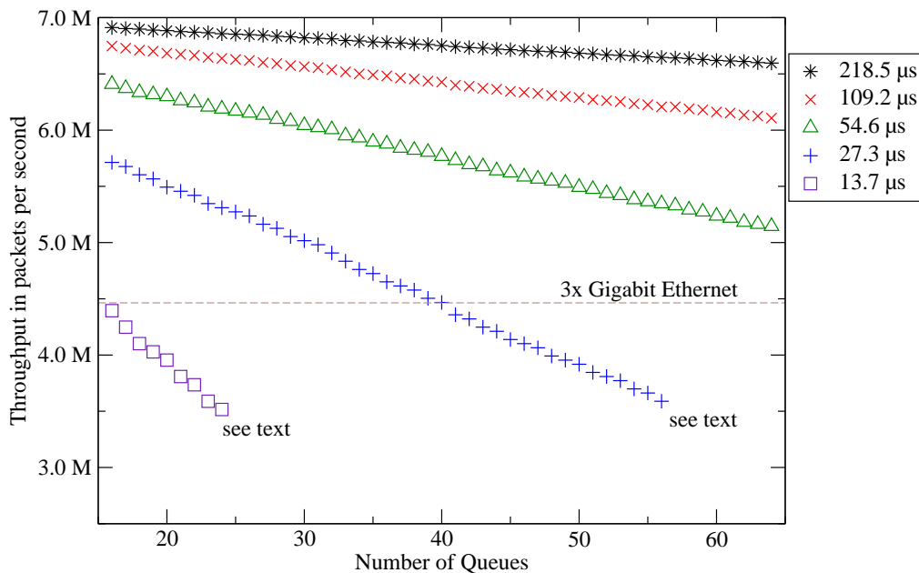
Fig. 8. Calculated throughput of the BAM for different timer granularities
