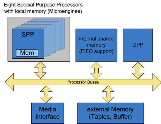
Fig. 3. Simplified architecture of the IXP2400
