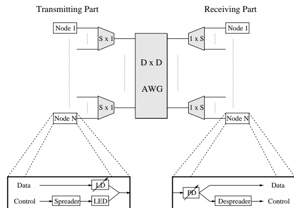
Fig 4.1 Architecture of a single hop network based on an Arrayed Waveguide Grating
