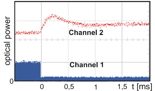
Fig. 2.3: Measured transient gain variation
