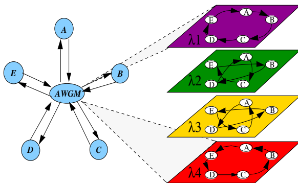
Fig. 4.2 Architecture of a multihop network based on an Arrayed Waveguide Grating
