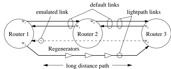
Fig 3.1 A unidirectional link with a tunnel
