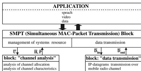
Fig. 2.5: Interface between physical and data link control layers
