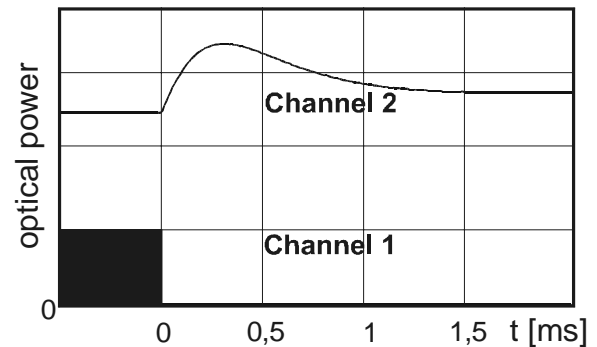
Fig. 2.4: Simulated transient gain variation
