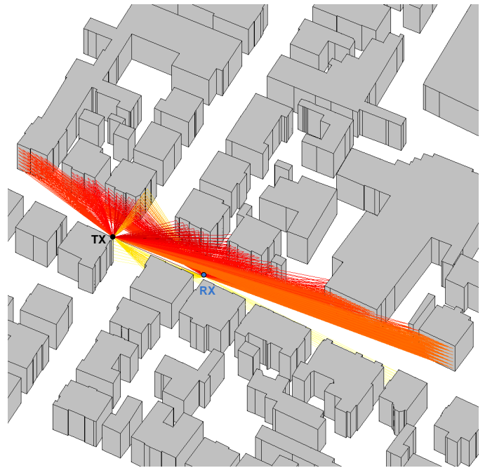
Figure 2: 3D-ray-optical model
